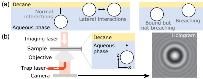
FIG. 1. (a) On the left is a schematic of the normal and lateral interactions and on the right a schematic of two ways in which particles can bind to the interface. (b) Diagram of the all-optical apparatus used to push a particle to an interface and capture holograms, which are used to measure the particle position in three dimensions.
