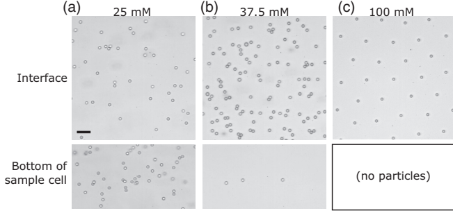
FIG. 11. Normal interactions depend on salt concentration. We prepare sample cells with (a) 25 mM, (b) 37.5 mM, or (c) 100 mM NaCl in the water phase. The unbound particles that settle to the bottom of the sample are shown in the bottom images. The scale bar is 10 \mu\text{m} .
