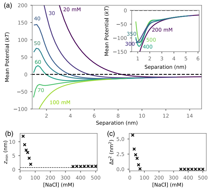
FIG. 7. A liquid-state theory predicts mean potentials between a polystyrene particle and an interface with the glycerol-water system on one side and decane on the other. The calculations reveal a potential well at 20–70 mM NaCl and above 325 mM NaCl (inset). (b) The position of the potential minimum z_{\min} decreases with increasing salt concentration, disappears, and then reappears at higher salt concentration. The ion diameter is shown by the dotted line. (c) The fluctuations of the particle in the well also decrease with salt concentration until the well disappears at about 70 mM. At concentrations above 325 mM, the well appears again.
