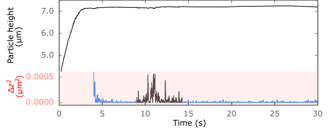
FIG. 9. Time-dependent binding of a polystyrene particle to an interface. The trajectory of a 1.9- \mu\text{m} -diam sulfate polystyrene particle that is pushed to an interface between the glycerol-water system and decane with radiation pressure. The particle binds to the interface at 5 s, unbinds at 9 s, and binds again at 14 s. Data were taken at 100 Hz.
