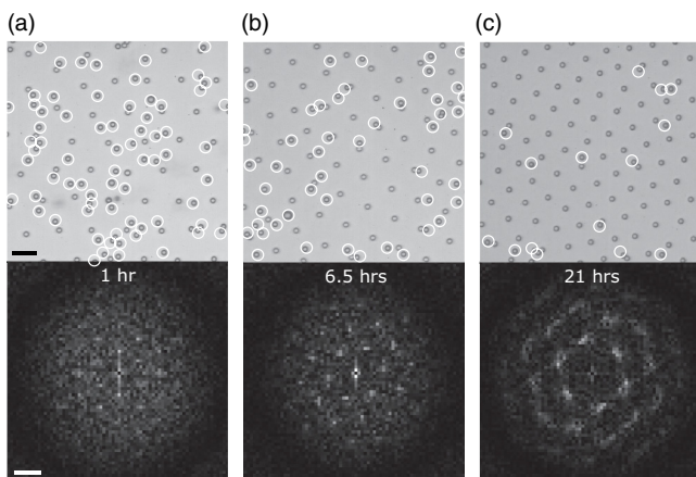
FIG. 6. The interface becomes more ordered over time, as particles that are bound without breaching eventually breach and become part of the crystal. The top row shows bright-field microscopy images of a 37.5 mM NaCl sample at (a) 1 h, (b) 6.5 h, and (c) 21 h after the sample is inverted. Particles that are bound without breaching are circled. The bottom row shows Fourier transforms of the top images, with the central DC pixel blocked to enhance contrast. Scale bars are 10 \mu\text{m} (top) and 0.1 \mu\text{m}^{-1} (bottom).
