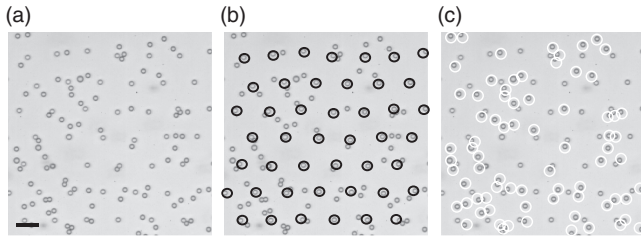
FIG. 5. Lateral interactions between particles breaching the interface appear unaffected by those that have bound without breaching. Panels show the same optical micrograph of particles at or near the interface in a sample with 37.5 mM salt. In (b) breaching particles are circled, showing that these particles have formed a crystal. The ordering is not readily apparent in (a). In (c) the particles that have bound without breaching are circled. Scale bar represents 10 \mu\text{m} .
