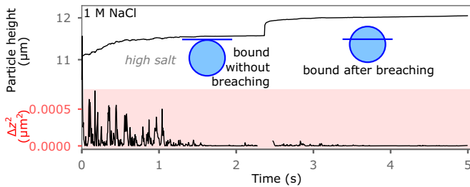
FIG. 3. Binding without breaching also affects particles at high salt concentrations before they breach. Top plot shows a 200-Hz trajectory of a 1.4- \mu\text{m} -diam particle in a 1 M NaCl aqueous solution. The reduction in fluctuations from the mean position averaged over a 0.2-s window (bottom plot) reveals that the particle binds to the interface at about 1.5 s without breaching it. The particle breaches the interface at around 2.5 s.
