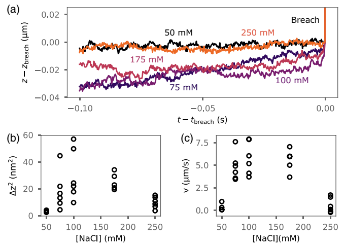
FIG. 4. Binding without breaching is reentrant with salt concentration. (a) The trajectories are of 2.0- \mu\text{m} -diam carboxyl latex particles and are taken at 4807.7 Hz. Here z_{\text{breach}} is the height of the particle in the frame just before the breach, which occurs at t_{\text{breach}} . (b) The fluctuations are calculated from a centered 0.2-s sliding average of z(t) . (c) The speed of the particle \Delta z/\Delta t is measured at \Delta t = 2.08 ms before the breach. The particles at the highest and lowest salt concentrations breach abruptly and have smaller fluctuations before breaching. Particles at intermediate concentrations have larger fluctuations and speeds before breaching.
