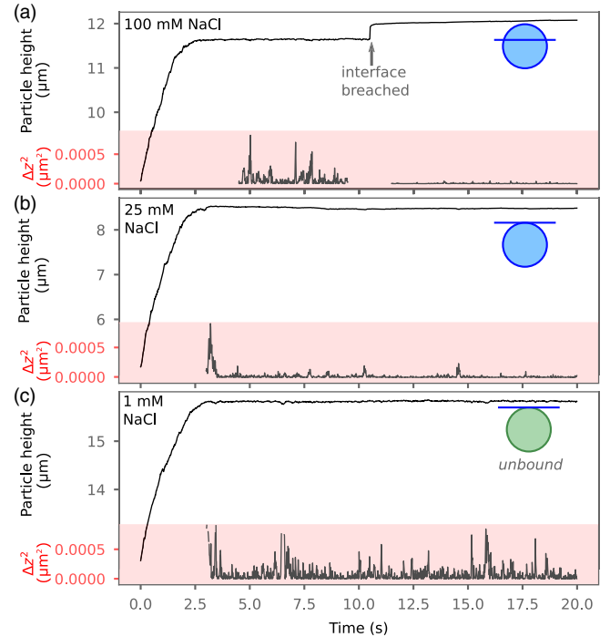
FIG. 2. Negatively charged polystyrene particles show three types of normal interactions. The upper plots show the height z of 1.9- \mu\text{m} -diam sulfate polystyrene particles (measured from the focal plane of the objective) as the particles move toward an interface between the glycerol-water system and decane under weak radiation pressure (data shown at 100 Hz). The lower plots show the fluctuations in height \Delta z^2 , defined as the square of the particle's displacement from its mean height at a given time t , as calculated from a centered sliding average with a 1-s window. (a) At moderate NaCl concentrations (100 mM), particles breach the interface (11 s). Because of the rapid movement of the particle during the breach, we do not show the fluctuations in this part of the trajectory. (b) At low NaCl concentrations (tens of mM), particles approach the interface and bind to it without breaching it. Binding is evidenced by the decrease in fluctuations at about 4 s. (c) At very low salt concentrations (less than 10 mM), particles approach the interface and do not bind, as evidenced by the large fluctuations.
