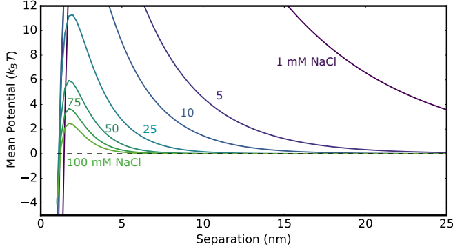
FIG. 12. The DLVO theory, modified to include effects of the interface, does not explain the observed interactions. The plot shows the mean potentials between a polystyrene particle and an interface with the glycerol-water system on one side and decane on the other as a function of salt concentration with zeta potential \zeta_p = -10 mV for the plane and \zeta_s = -55 mV for the particle.
