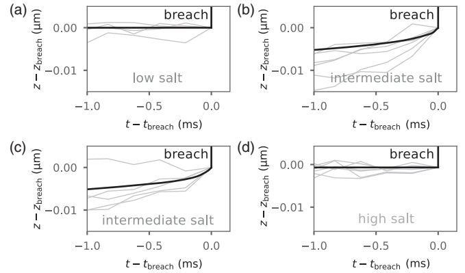
FIG. 8. Trajectories of particles prior to breaching agree with model predictions. Measured trajectories are shown in gray and trajectories calculated from our model in black. (a) At low salt concentration (50 mM), particles bind to the interface before breaching. (b) At moderate salt concentrations (100 mM), particles breach the interface without binding first. Furthermore, they accelerate toward the interface before breaching. (c) Behavior similar to that in (b) but for 175 mM NaCl in experiment and 200 mM in calculations. At high salt concentrations (250 mM NaCl in experiment and 350 mM NaCl in calculations), particles bind to the interface before breaching and no acceleration is seen.
